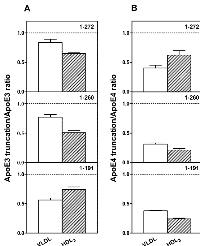
FIGURE 2: Effects of C-terminal truncations on the ability of apoE3 and apoE4 to bind to VLDL and HDL 3 : (A) apoE3 C-terminal truncation mutants/apoE3 and (B) apoE4 C-terminal truncation mutants/apoE4. The results from two to five independent experiments, each conducted in triplicate, are reported as means \pm SD.
