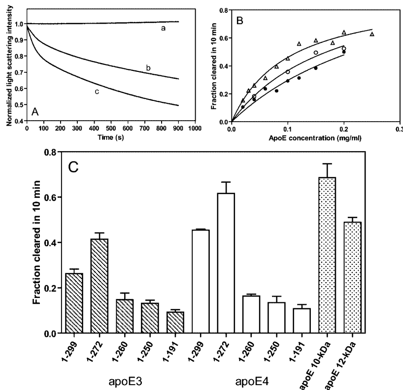
FIGURE 9: Solubilization of DMPC multilamellar vesicles by apoE C-terminally truncated mutants. (A) Time courses for turbidity clearance: DMPC alone (a), apoE3 (b), and apoE4 (c). The DMPC and protein concentrations were 0.25 and 0.1 mg/mL, respectively. (B) Effect of protein concentration on fraction cleared in 10 min: apoE3 (●), apoE4 (Δ), and apoE4(E255A) (○). (C) Comparison of DMPC solubilization efficiency. The protein concentration was 0.1 mg/mL. The results from three to five independent experiments using different batches of protein are shown.
