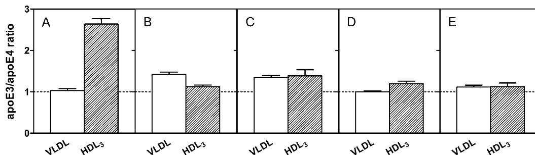
FIGURE 1: Effects of C-terminal truncation of apoE3 and apoE4 on the relative distributions between VLDL and HDL 3 . The apoE variants were incubated at 4 °C for 30 min with a mixture of human HDL 3 and VLDL. For ease of comparison, the ratios for the initial mixtures are normalized to 1 in each case: (A) apoE3/apoE4, (B) apoE3 (1–272)/apoE4 (1–272), (C) apoE3 (1–260)/apoE4 (1–260), (D) apoE3 (1–250)/apoE4 (1–250), and (E) apoE3 (1–191)/apoE4 (1–191). The results from two to five independent experiments, each conducted in triplicate, are reported as means \pm SD.
