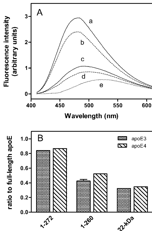
FIGURE 5: ANS fluorescence for apoE3 C-terminally truncated mutants. (A) Emission spectra of ANS in the presence of apoE3 (a), apoE3 (1–272) (b), apoE3 (1–260) (c), 22 kDa apoE3 (d), and buffer (e). (B) ANS fluorescence intensity ratio of the C-terminally truncated mutants to full-length apoE. The results from at least two independent experiments, each conducted in triplicate, are shown.
