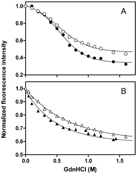
FIGURE 8: GdnHCl denaturation of single-Trp mutants of apoE3 and apoE4 monitored by Trp fluorescence. Normalized fluorescence intensity at 335 nm was plotted as a function of GdnHCl concentration: (A) apoE3 W@264 (○) and apoE4 W@264 (●) and (B) apoE3 (1–272) W@264 (△) and apoE4 (1–272) W@264 (▲). The results from two to three independent experiments, each conducted in duplicate, are shown.
