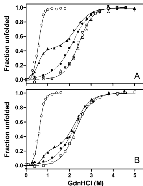
FIGURE 4: GdnHCl denaturation of full-length apoE3, 22 and 10 kDa fragments of apoE3, and C-terminally truncated apoE3 monitored by Trp fluorescence (A) and CD (B): full-length apoE3 ( \blacktriangle ), apoE3 (1–272) ( \bullet ), apoE3 (1–260) ( \triangle ), apoE3 (1–250) ( \nabla ), 22 kDa apoE3 ( \square ), and 10 kDa apoE3 ( \circ ).
