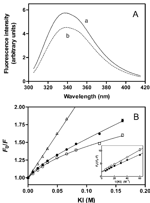
FIGURE 7: Fluorescence spectroscopy of apoE3 and apoE4 single-Trp mutants. Solutions of the proteins (100 \mu\text{g}/\text{mL} ) were excited at 295 nm to obtain the emission fluorescence from W264. (A) Fluorescence spectra for apoE3 W@264 (a) and apoE4 W@264 (b). (B) Stern–Volmer plot comparing quenching by KI of W264 fluorescence from apoE3 (○) and apoE4 (●). The data for N -acetyltryptophanamide are also shown for comparison (△). The inset shows a modified Stern–Volmer plot. The results from two to four independent experiments, each conducted in triplicate, are shown.
