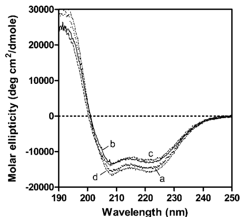
FIGURE 3: Far-UV CD spectra of apoE3 C-terminally truncated mutants: apoE3 (a), apoE3 (1–272) (b), apoE3 (1–260) (c), and 22 kDa apoE3 (d). The protein concentration was 50 \mu\text{g/mL} .
