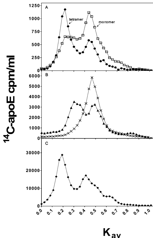
FIGURE 6: Elution profiles upon gel filtration of apoE3 and apoE4 variants on a Superdex 200 column. Proteins at a concentration of 5 \mu g/mL (A and B) or 50 \mu g/mL (C) were subjected to gel filtration: (A) full-length apoE3 (●) and full-length apoE4 (□), (B) apoE3 (1–272) (▲) and apoE4 (1–272) (×), and (C) apoE4(E255A) (◆). Representative profiles from at least three independent experiments using different batches of protein are shown.
